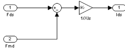
Figure 37. Ids matlab simulink block. block sub-system.
