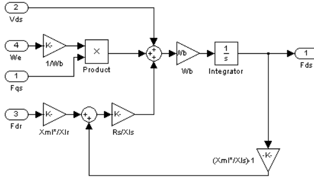
Figure 21. Fds matlab simulink block
