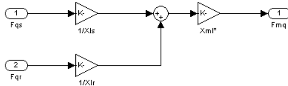
Figure 29. Fmq matlab simulink block.
