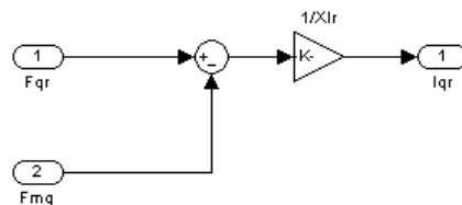
Figure 31. Iqr matlab simulink block.
