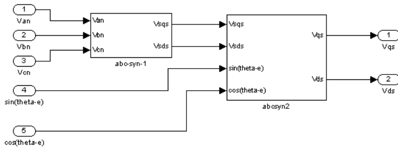
Figure 10. abc-syn conversion simulink block.
