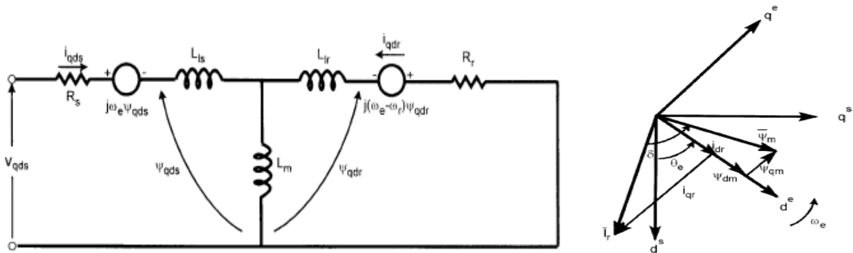
Figure 4. Complex synchronous frame dqS equivalent circuit.
