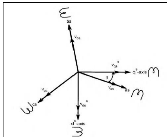
Figure 1. Stationary frame (as-bs-cs to d^s - q^s ) axes transformation
