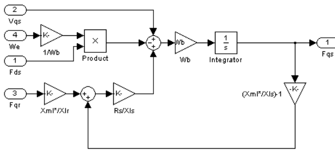
Figure 25. Fqs matlab simulink block sub-system
