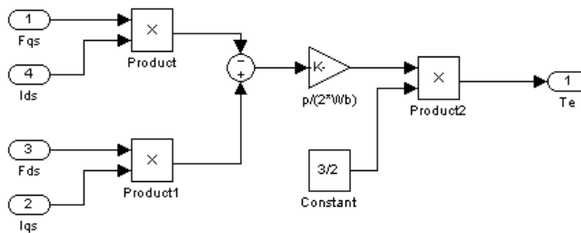
Figure 39. Te matlab simulink block. block sub-system.
