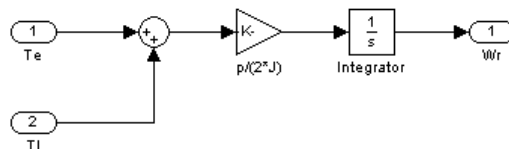
Figure 41. \omega_r matlab simulink block. block sub-system.
