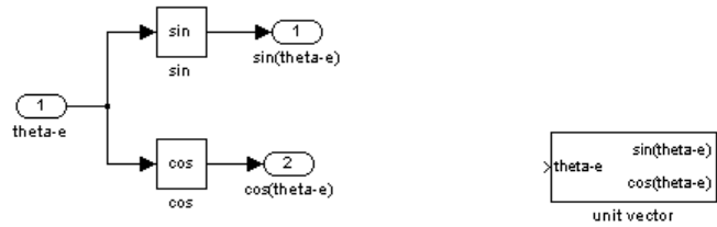
Figure 9. Unit vector simulink block.
