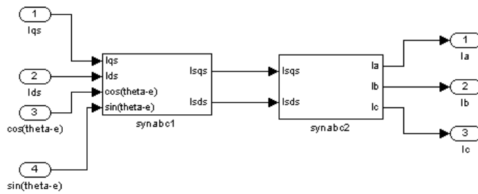
Figure 14. Syn-abc conversion simulink block
