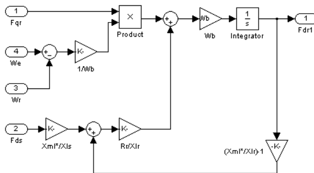
Figure 19. Fdr simulink block sub-system.
