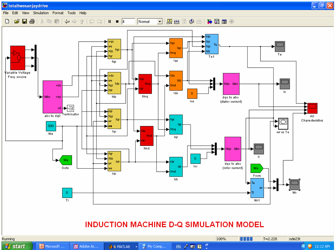
Figure 44. Induction machine D-Q simulink model.
